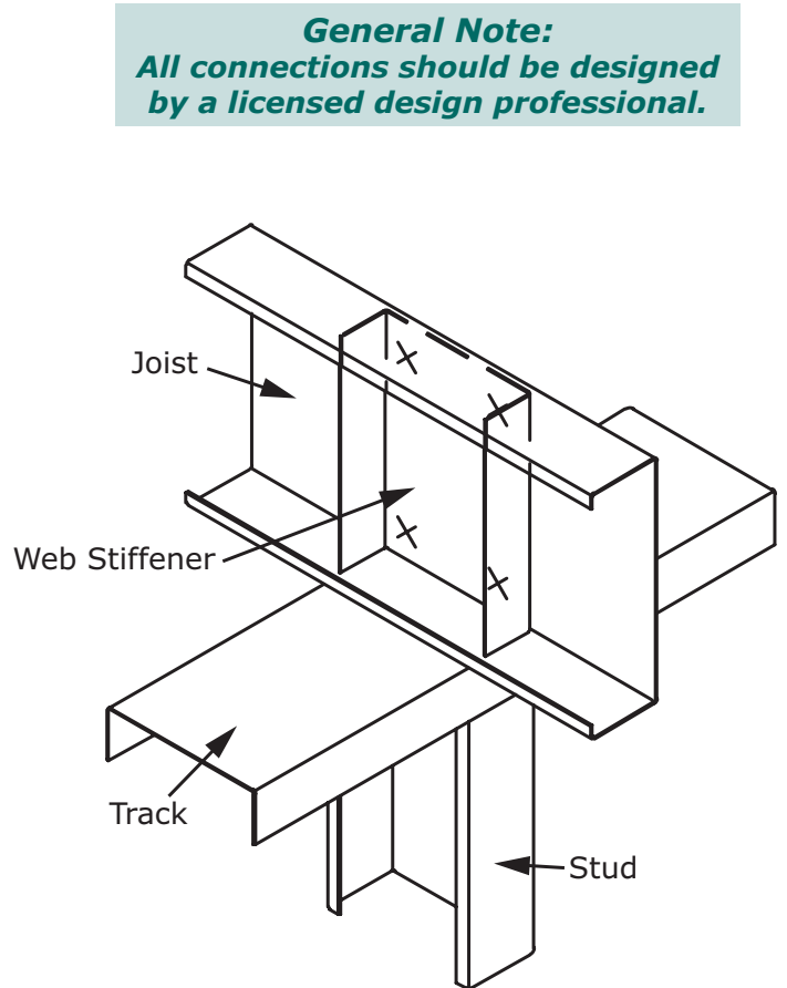
Track Stiffener Inside Joist
